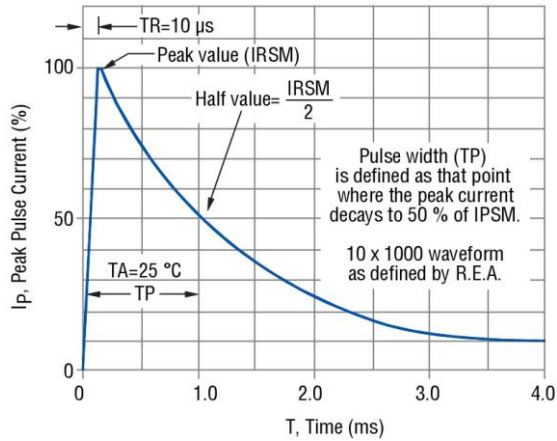
Figure 3 - Pulse Waveform
